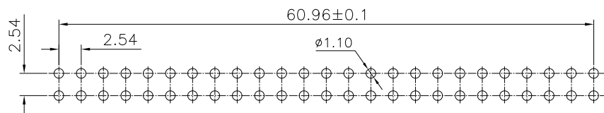
PCB Layout
