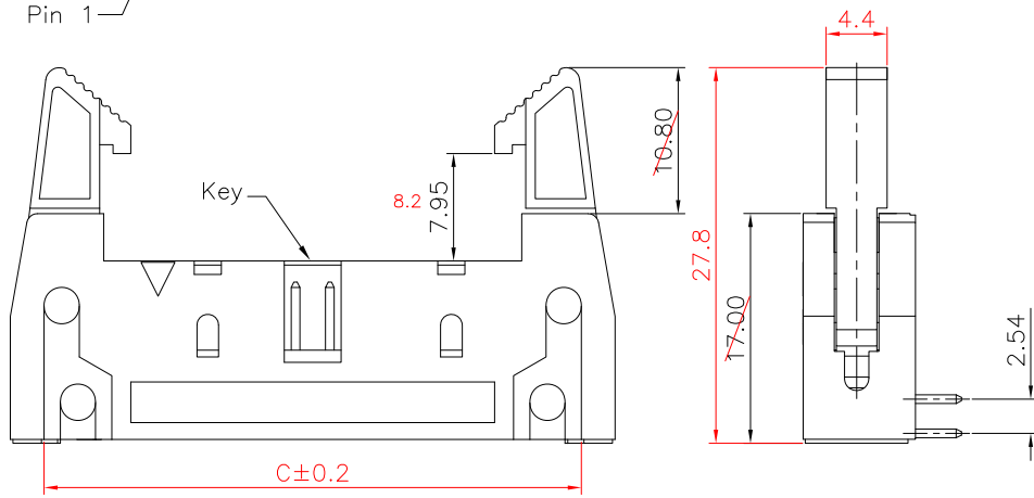
MATING PART 3030-XX-0103-00
